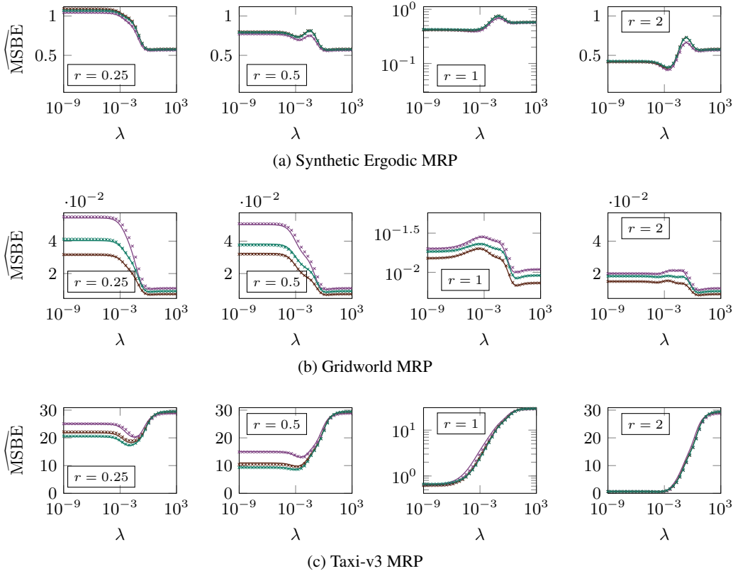
Figure 11: MSBE is not an increasing function of the l_2 -regularization parameter \lambda . Continuous lines indicate the theoretical values of \widehat{\text{MSBE}} from Theorem 5.2 for n = 1000 (purple), n = 3000 (maroon), and n = 5000 (green); the crosses are numerical results averaged over 30 instances after the learning with regularized LSTD in synthetic ergodic, Gridworld and Taxi-v3 MRPs for d = 50, n = 3000, d = 50, n = 5000 and d = 50, n = 5000 , respectively. Note that the y-axis has a logarithmic scale for r = N/m = 1 .
